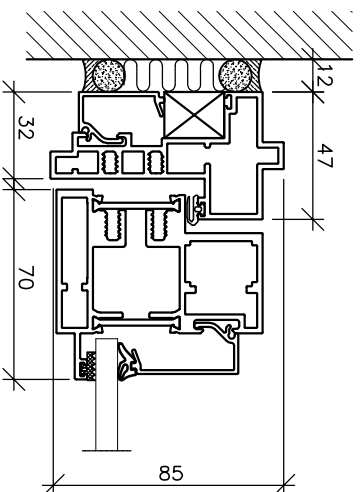
1. Samling glas/loft
